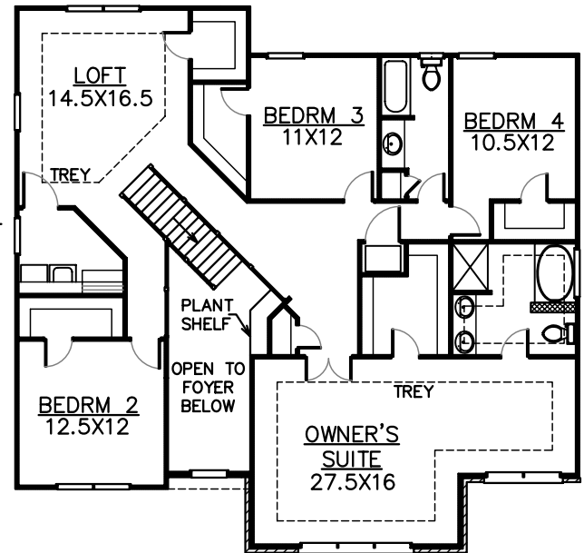
SECOND FLOOR 1943 FINISHED SQ. FT.
